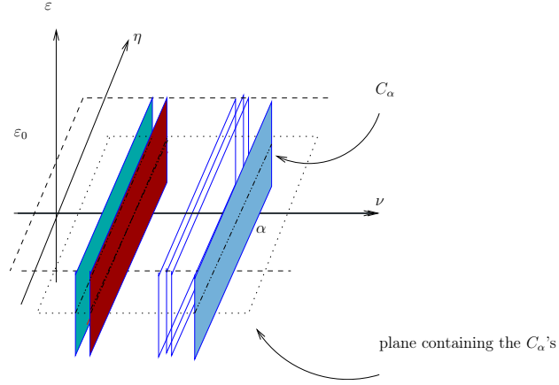
FIGURE 1. The Cantor set of surfaces: transversely cutting with a plane \varepsilon = \text{const} we obtain the Cantor set of curves like the one described in theorem 3.2
